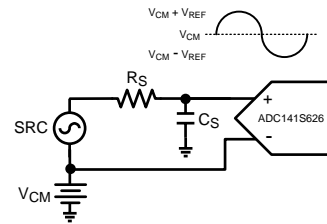
Figure 40. Single-Ended Input
